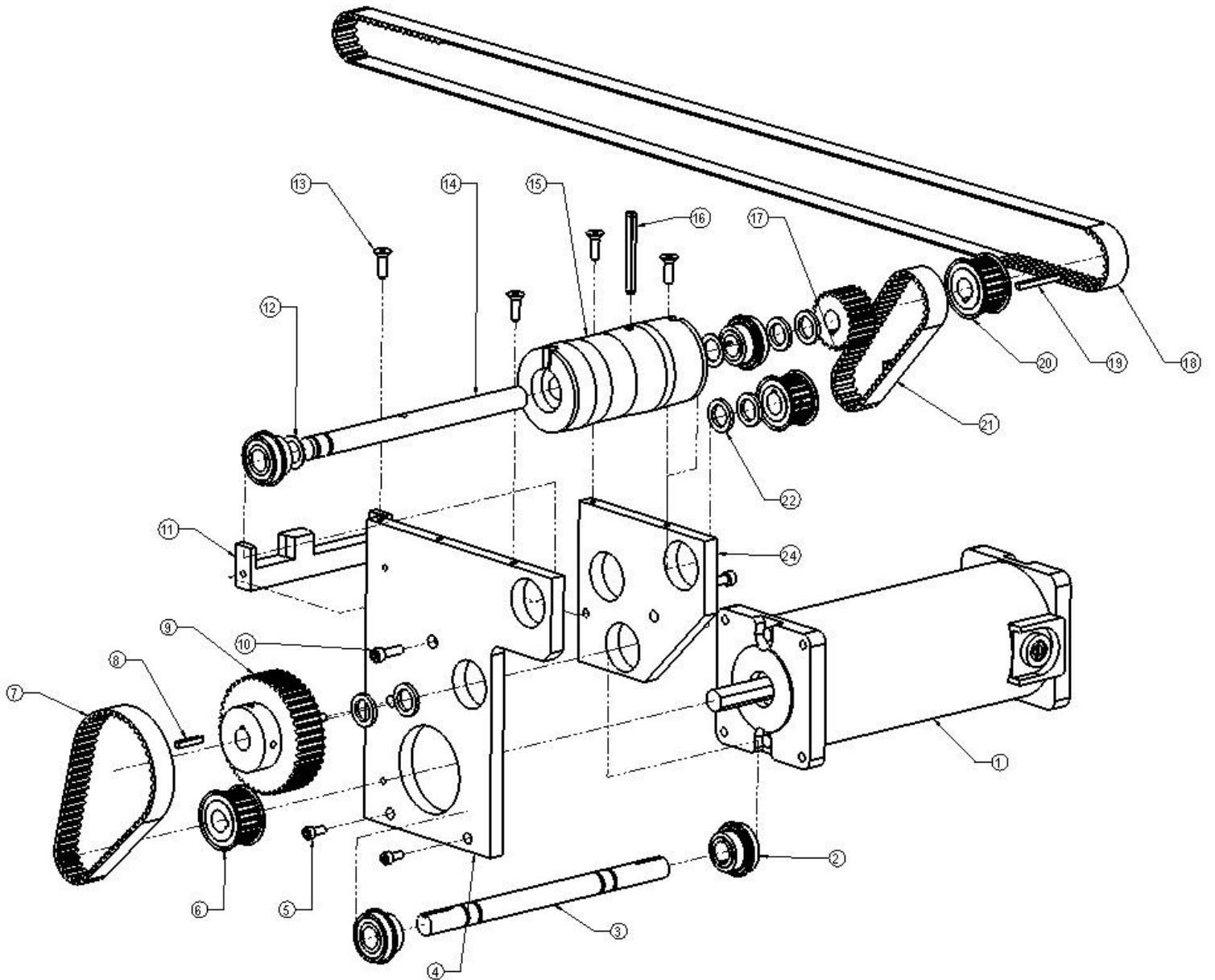
FIG. 3 Assembly Drive Output Ext.
